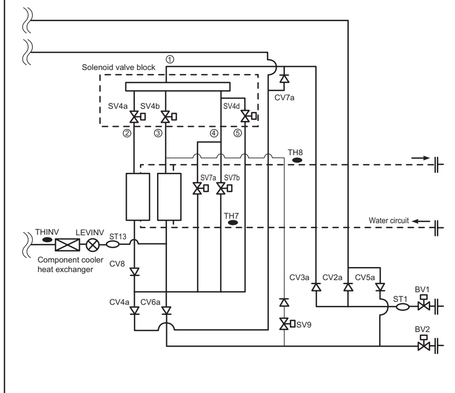
Solenoid valve block(three compartments)
