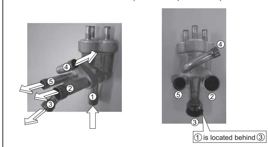
Solenoid valve block(three compartments)
