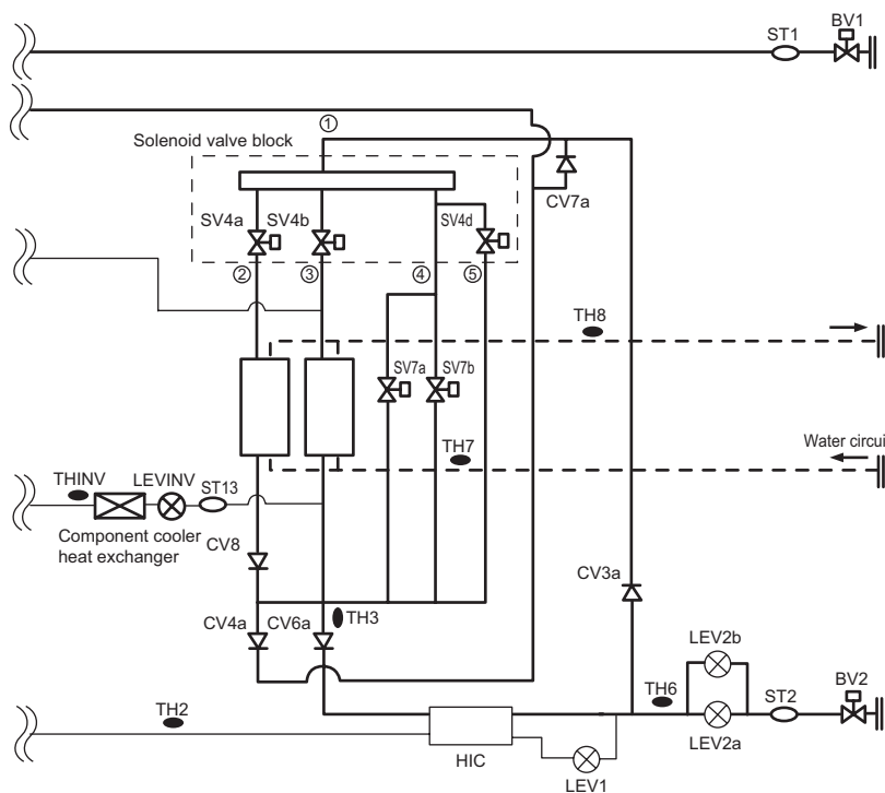
Refrigerant Circuit diagram <PQHY>
